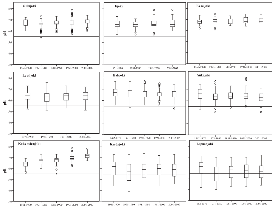
Fig. 4. Median, upper and lower 25th percentiles and minima and maxima for pH in the nine rivers studied in Paper I, 1961–2007. The critical value of pH in ecological classification, 5.5 is indicated by a horizontal line (I, published by permission of Elsevier).
