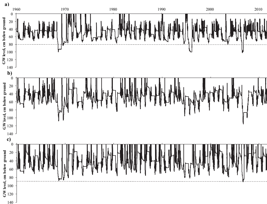
Fig. 8. Simulated GW level at (a) site 1, (b) site 2 and (c) site 3 in the period 1960–2011. Boundary between peat and mineral horizons marked as a horizontal dashed line. At site 2, the boundary is at 160 cm depth (V, published by permission of Elsevier).
